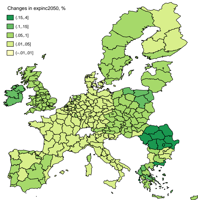
Figure 14: Simulation results of an asymmetric (TEN-T) multi-region integration shock: Long-run (2050) impacts of improvement in regions' accessibility on expected income , changes percent. Simulations are performed using the RHOMOLO v.2 model.
