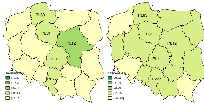
Figure 7: Simulation results of a symmetric multi-region (PL11, PL12, PL22, PL61 and PL63) integration shock. Short-run (2010, left figure) and long-run (2050, right figure) impacts of improvement in regions' accessibility on real wages , changes in percent. Simulations are performed using the RHOMOLO v.2 model with all NUTS2 regions in EU-27, reported are only the Polish regions (the impact on other EU regions is of lower order of magnitude).
