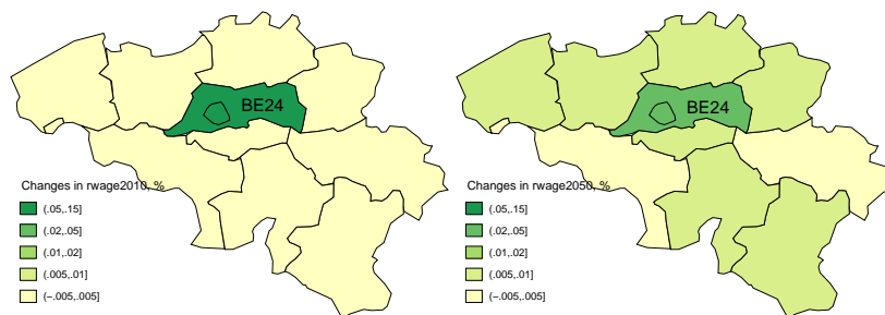
Figure 3: Simulation results of a symmetric single region (BE24) integration shock. Short-run (2010, left figure) and long-run (2050, right figure) impacts of 10 % improvement in region’s accessibility on real wages , changes in percent. Simulations are performed using the RHOMOLO v.2 model with all NUTS2 regions in EU-27, reported are only the Belgian regions (the impact on other EU regions is of lower order of magnitude).
