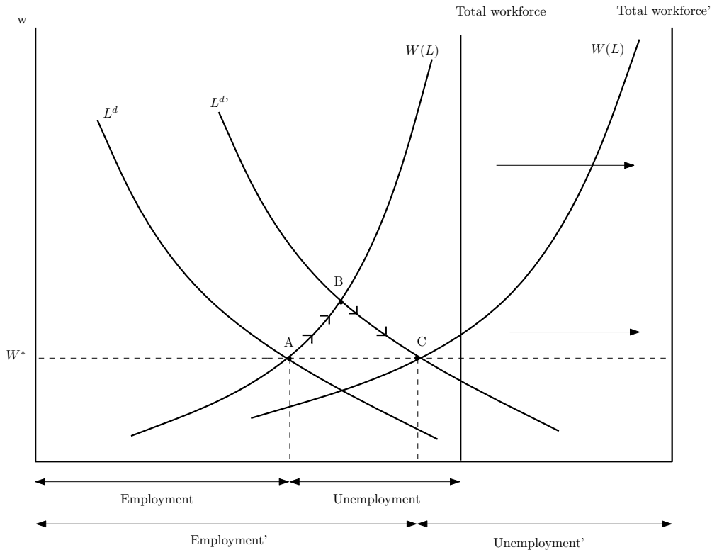
Figure 1: An illustration of the partial equilibrium effect of a single shift in labour demand (A→B), and subsequent in-migration (B→C), on regional wages, employment and unemployment. The shift has a temporary effect on wages and the unemployment rate, and a permanent effect on the size of the local labour force.
