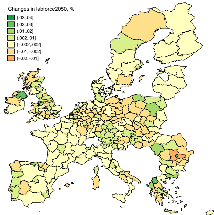
Figure 15: Simulation results of an asymmetric (TEN-T) multi-region integration shock: Long-run (2050) impacts of improvement in regions' accessibility on labour force , changes in percent. Simulations are performed using the RHOMOLO v.2 model.
