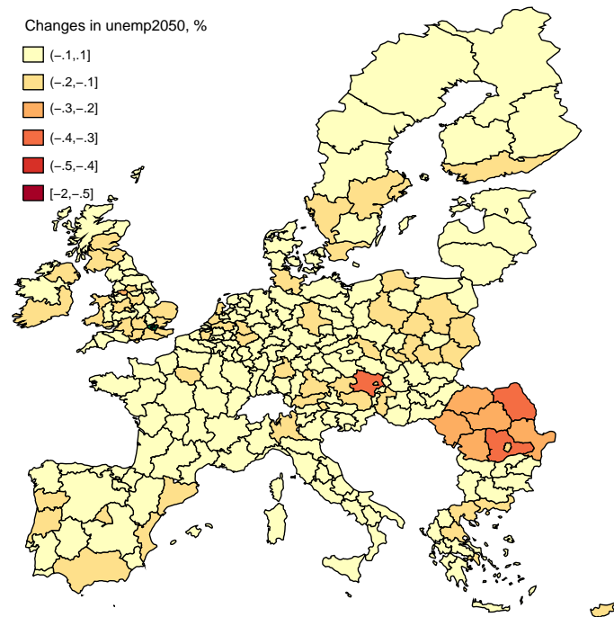
Figure 13: Simulation results of an asymmetric (TEN-T) multi-region integration shock: Long-run (2050) impacts of improvement in regions' accessibility on unemployment , changes in percent. Simulations are performed using the RHOMOLO v.2 model.
