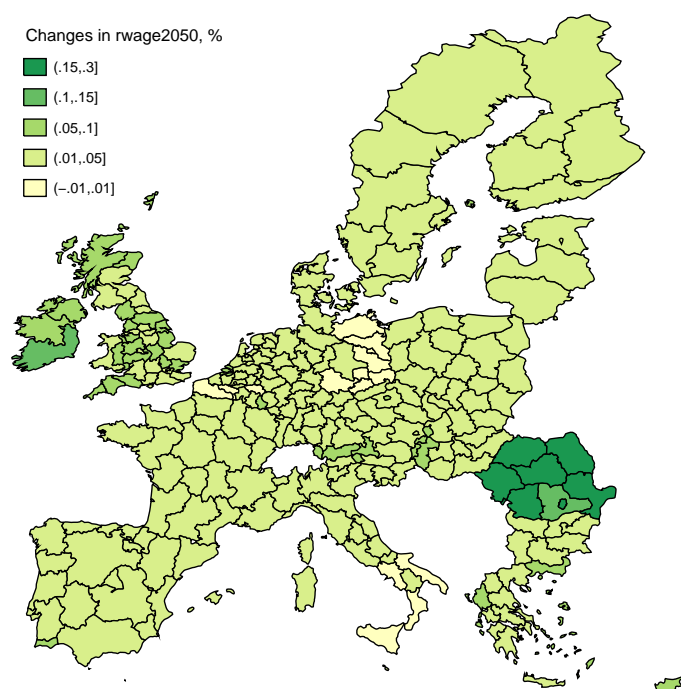
Figure 12: Simulation results of an asymmetric multi-region integration shock: Long-run (2050) impacts of improvement in regions' accessibility on real wages , changes in percent. Simulations are performed using the RHOMOLO v.2 model.
