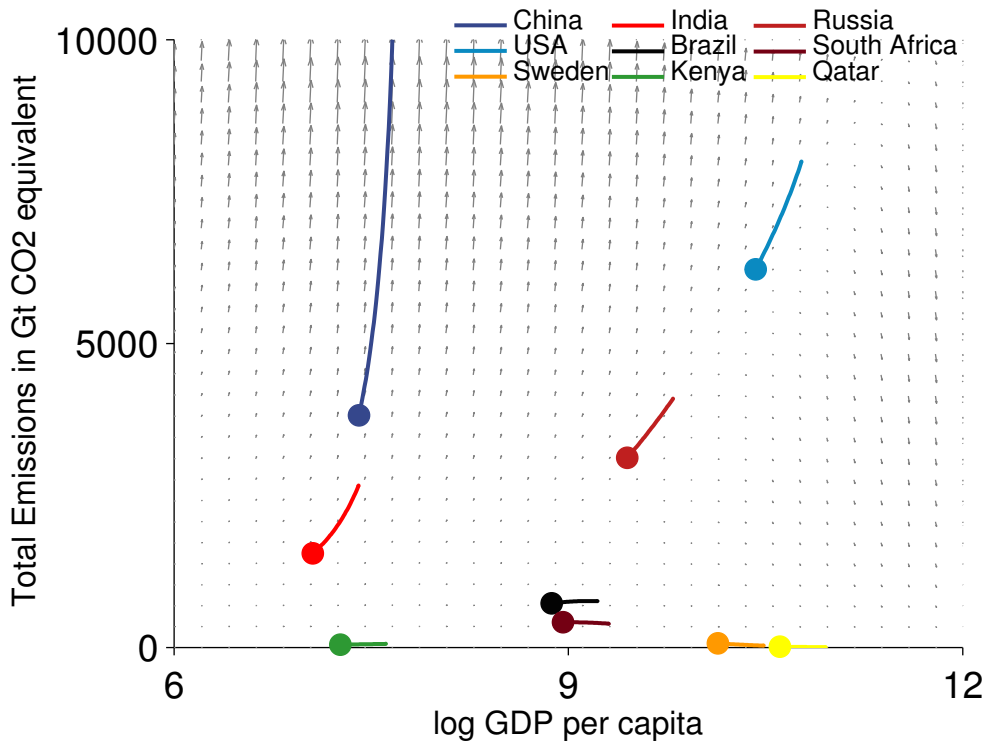
Figure 2. : The model predictions for total emissions against log GDP per capita for all countries from 1990-2005. The coloured vector lines show the predicted country trajectories starting from 1990 initial conditions for the same time period.
