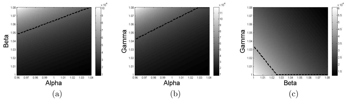
Figure 5. : Predicted total global emissions in 2020 shown as a function of changing two of the parameters \alpha , \beta and \gamma while keeping the third parameter constant at 1. The mapping of colour to amount of emissions is shown as a colourbar in units of tonnes of CO_2 equivalent. The dashed line in each sub-figure represents the desired target of 44 Gt CO_2 e.
