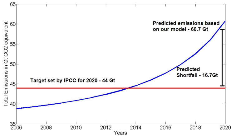
Figure 3. : Predicted Total Emissions with the IPCC target for 2020 to keep global temperature increase below 2 degrees C
