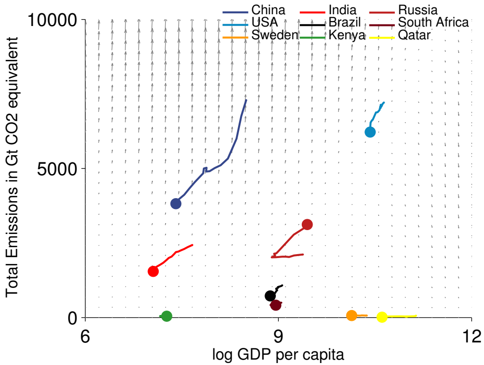
Figure 1. : Total emissions against log GDP per capita for all countries from 1990-2005. The black vector lines show the average yearly changes (magnitude and direction) in log GDP and total emissions as a function of current log GDP and total emissions. The coloured vector lines show representative country trajectories in the same time period.
