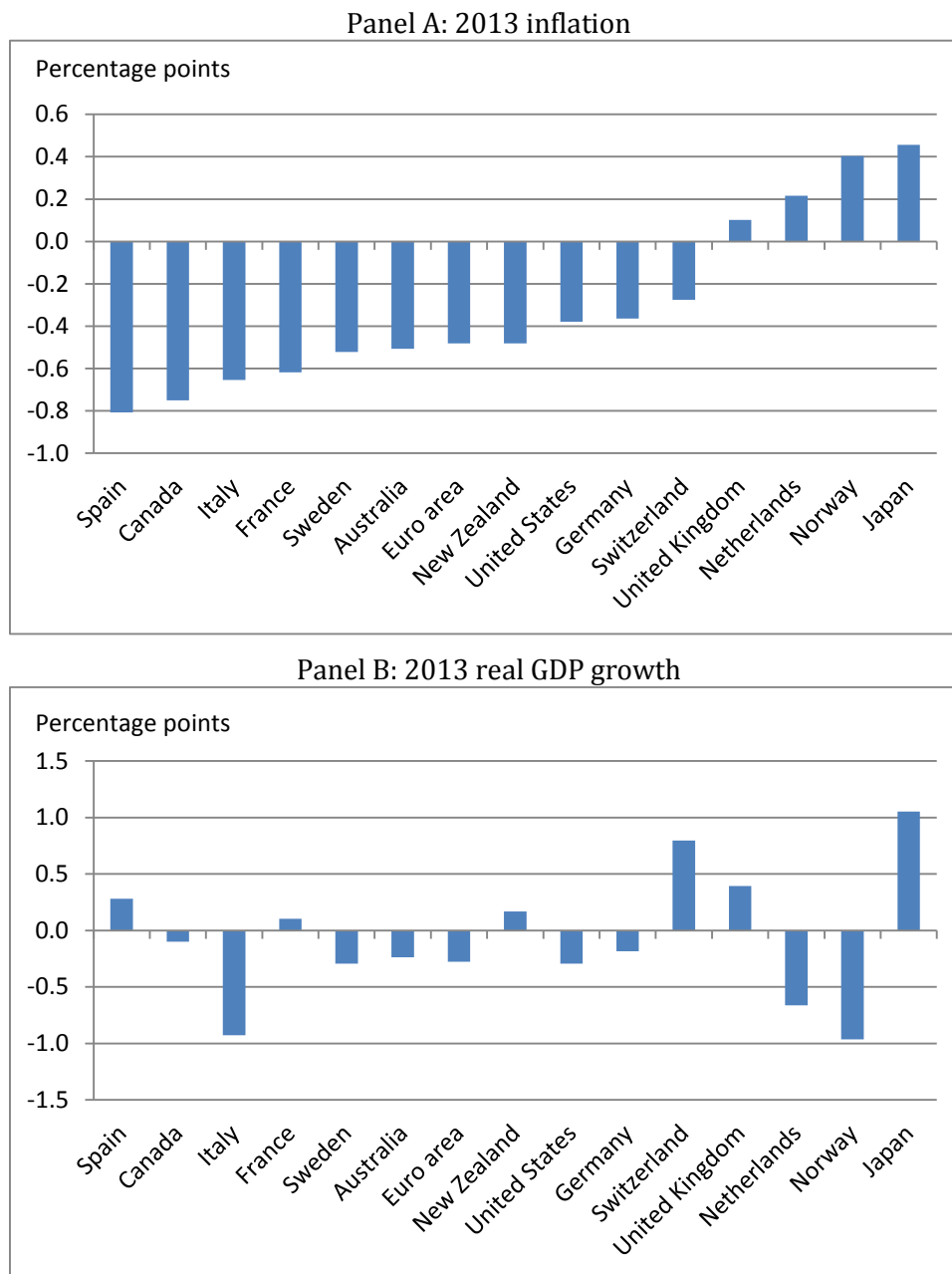
Figure 1: 2013 forecast revisions
