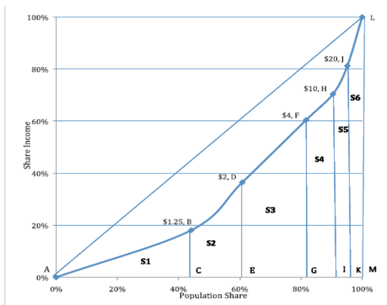
Graph 2 : Lorenz curve
