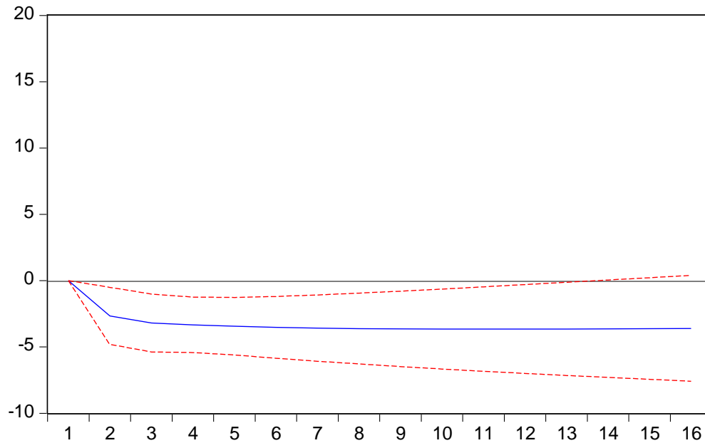
Response of INFLATION to DBACBA
