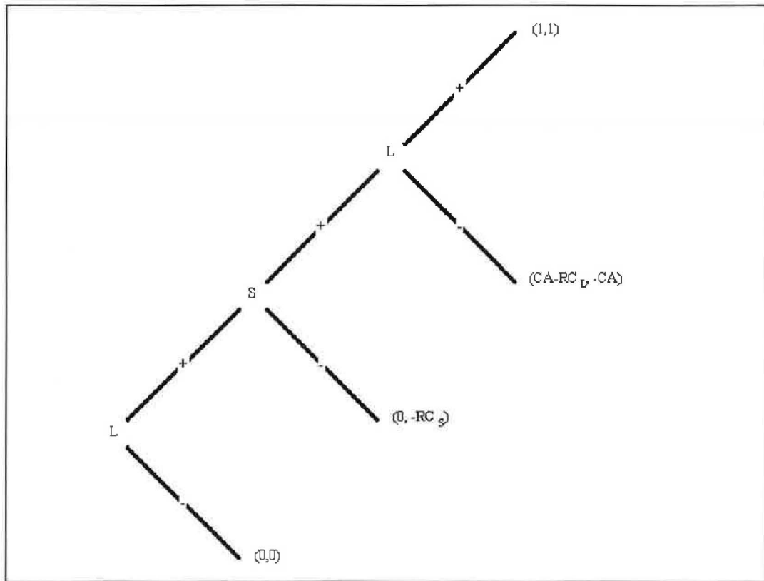
GRAPH 1: Decision Tree
