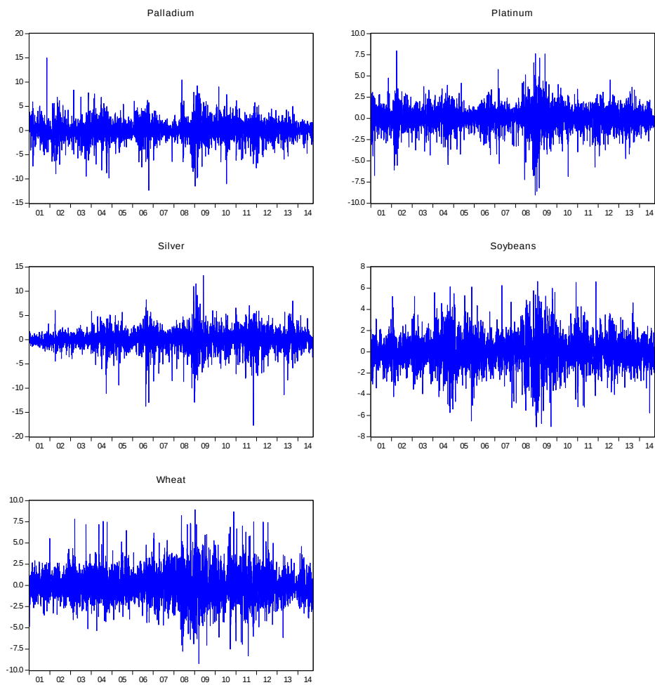
Figure 2: Commodity Returns
