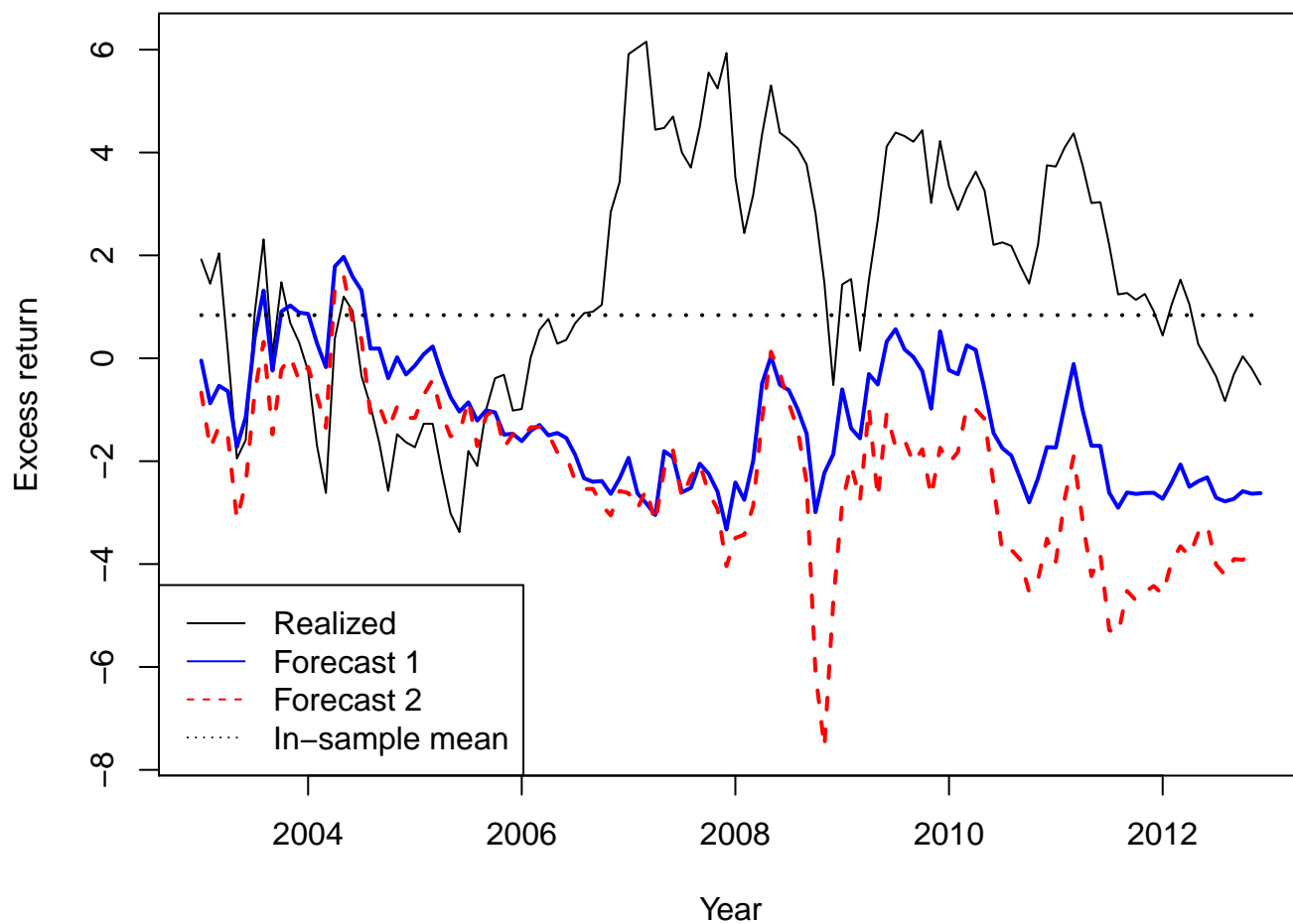
Figure 3: Cochrane-Piazzesi: out-of-sample forecasts
