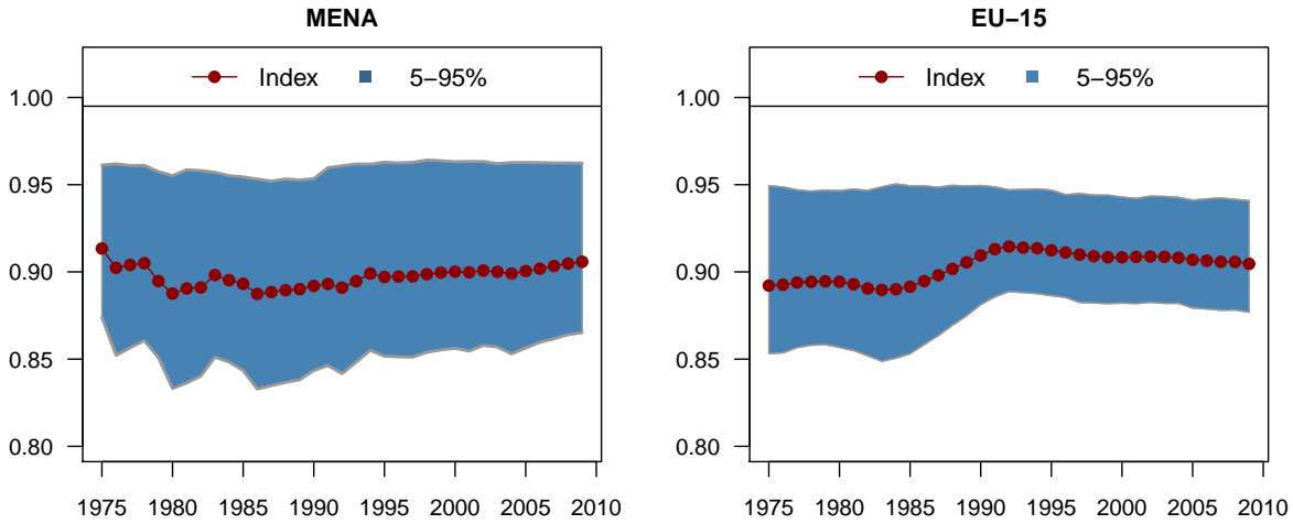
Figure 7: Integration measure I_E with estimated confidence bounds.
