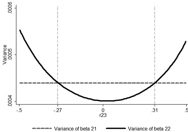
Figure 1. Monte Carlo Simulations
