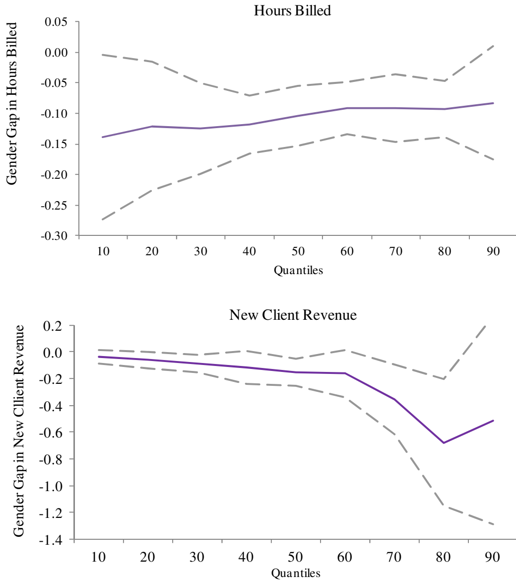
FIGURE 2 – PERCENTILES OF THE GENDER GAPS IN PERFORMANCE
