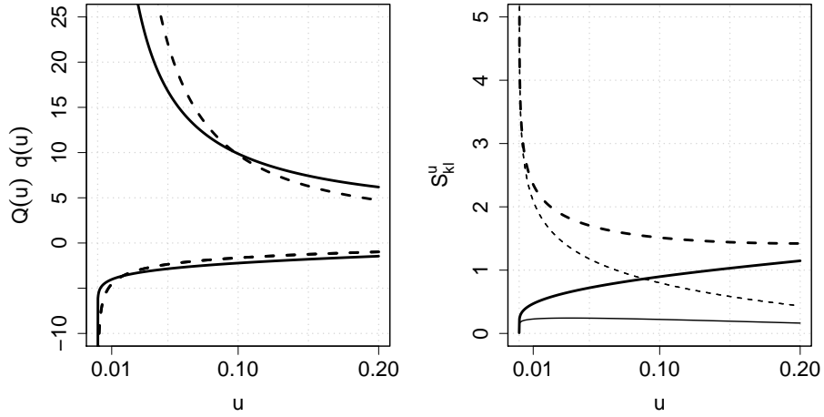
Figure 2.1: The left panel shows quantile function Q(u) (bottom) and quantile density function q(u) (top) for N(0,3) (solid) and t_3 (dashed). The right panel presents S_{\ell k}^{u_k} (dashed) for \alpha = 0.0001 (thin) and \alpha = 0.5 (thick).
