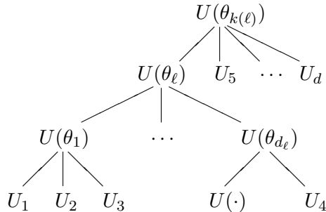
Figure 3.2: Example of a partially nested HAC.
