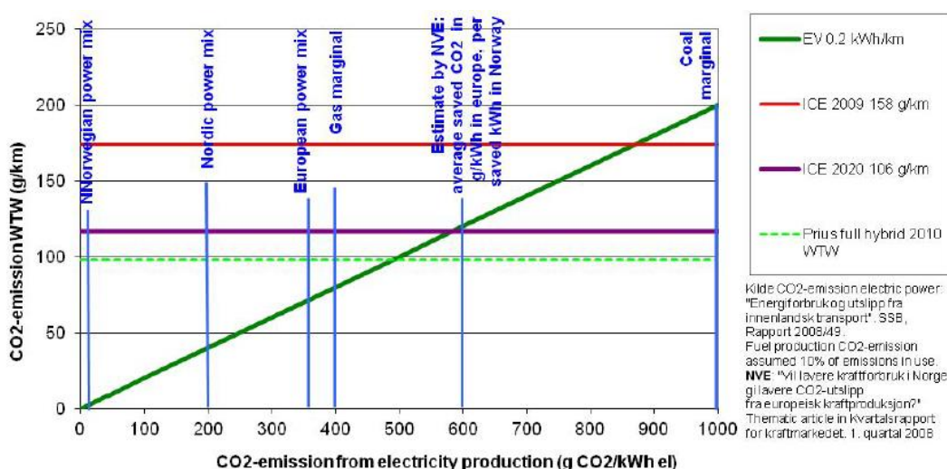
Figure 1. CO 2 emissions from electricity production
