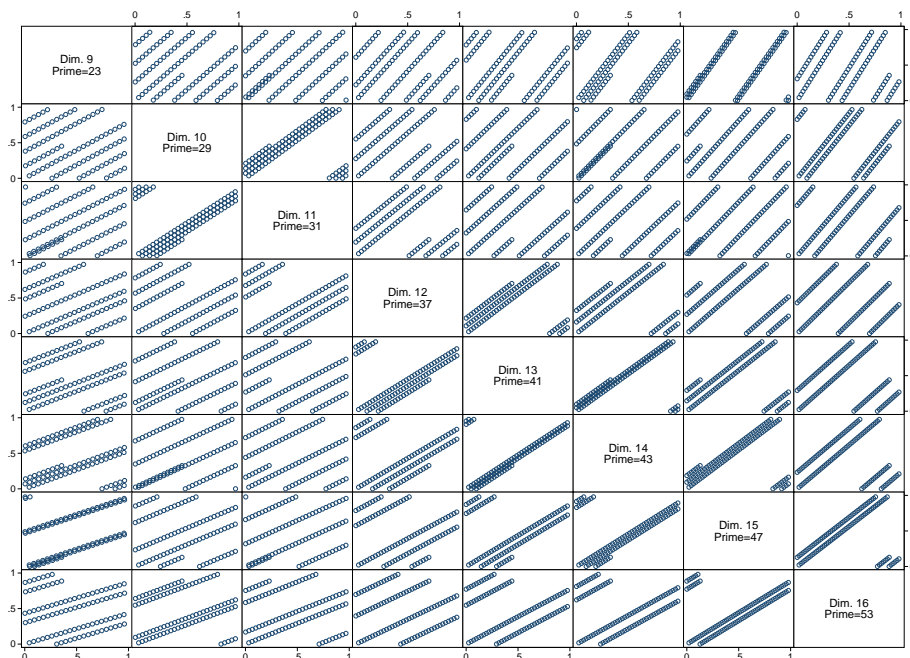
Figure 2: Scatter-plot matrix of two-dimensional Halton sequences with 100 points from dimension 9 (prime 23) to dimension 16 (prime 53)
