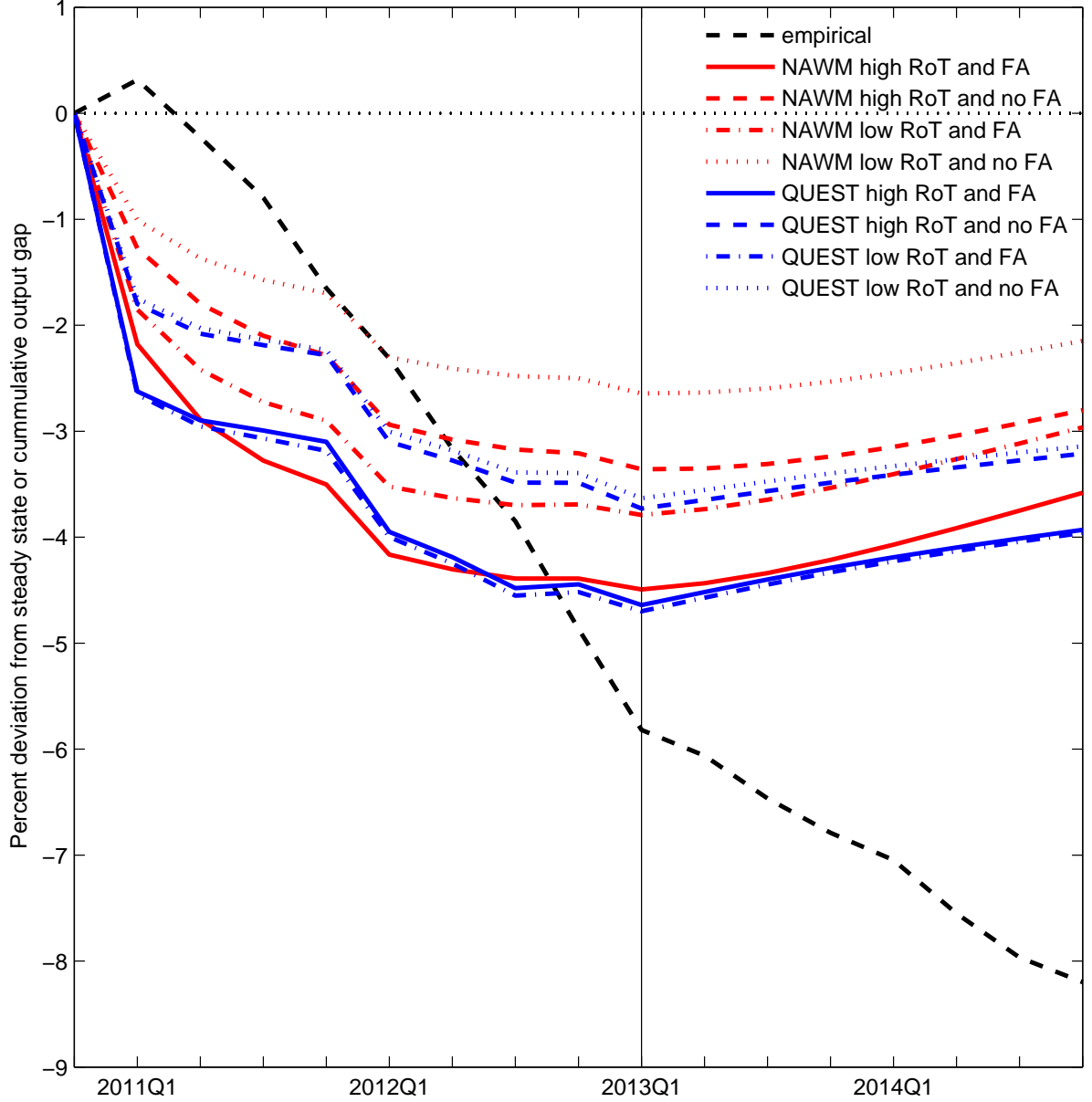
Figure 7: Output gap in the two models in the baseline setup and in the Euro Area (dashed line) since 2011Q1. We assume that the output gap in the data evolves as GAP_t - GAP_{t-1} = g_t^y - g^{yp} , where g_t^y and g^{yp} denote actual and potential quarterly GDP growth, respectively. We set g^{yp} equal to the average quarterly GDP growth rate over the pre-crisis (i.e. 1999-2007) period, i.e. 0.6%. The vertical line denotes the end of the last quarter of the EA's recession.
