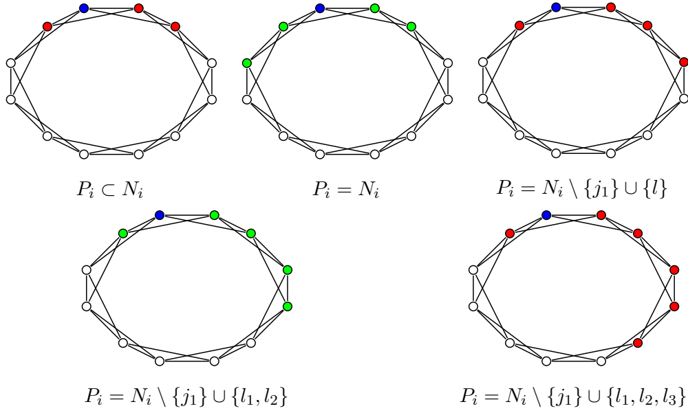
Fig. 5.1: Different scenarios in a circle network. Green nodes represent a WRP punishing set.
