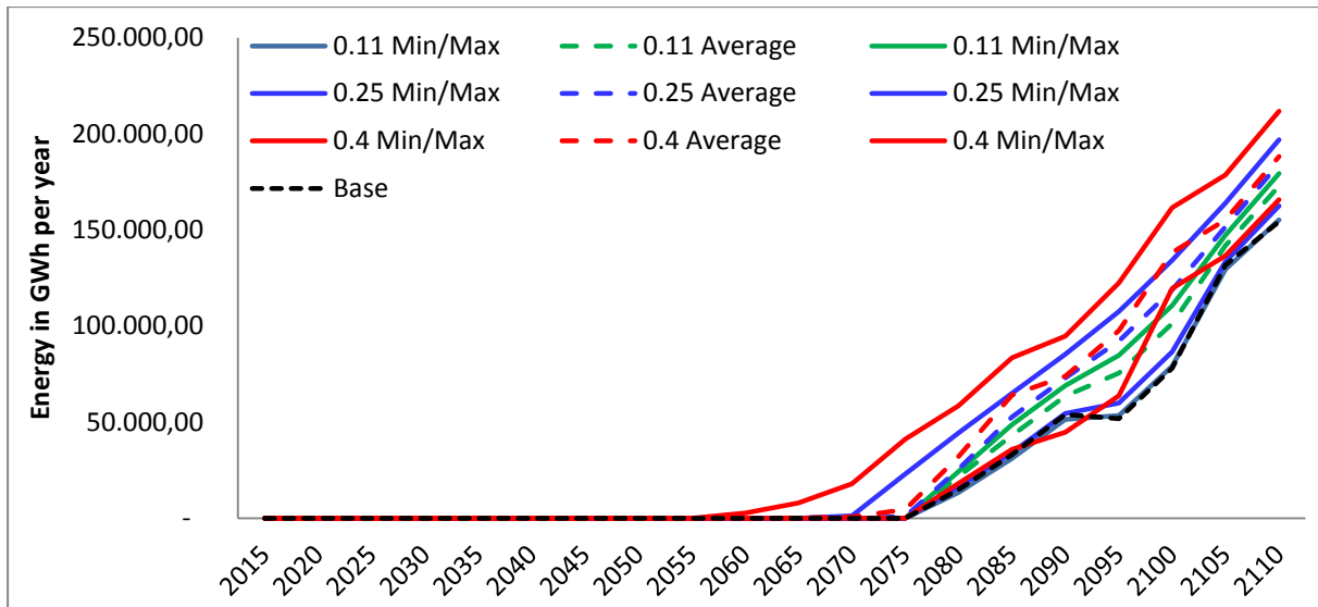
Figure 7E: Effects of water availability variability (using standard deviations of 0.11, 0.25 and 0.4) on solar energy production over time, annual electricity demand growth rate of 9%, Ethiopia energy sector model (GWh/year)
