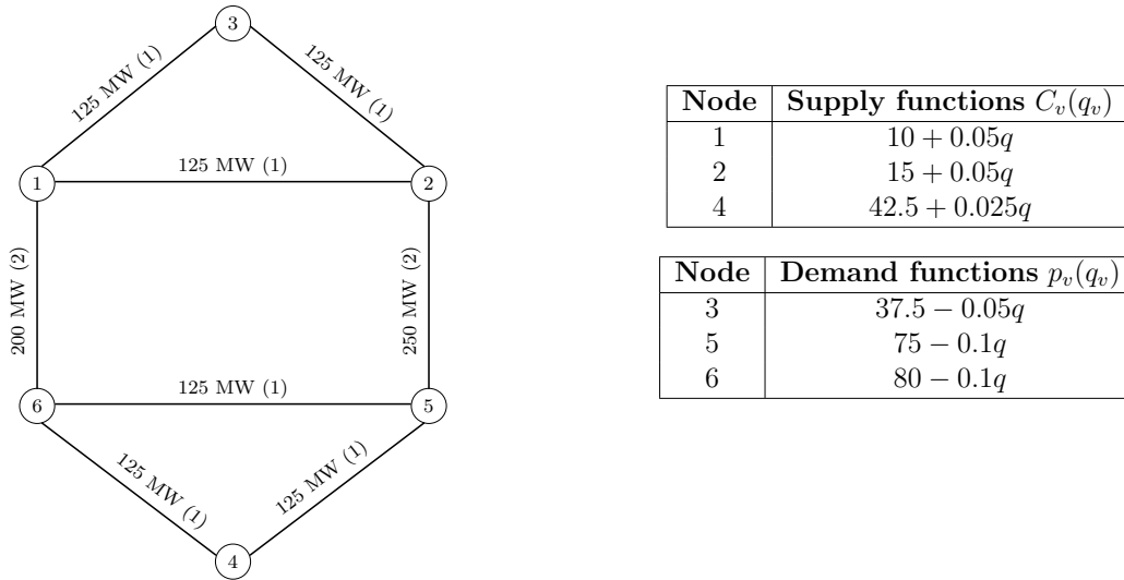
Figure 5: Basic spot market model (Chao and Peck, 1998), taken from de Maere d’Aertrycke and Smeers (2013)
