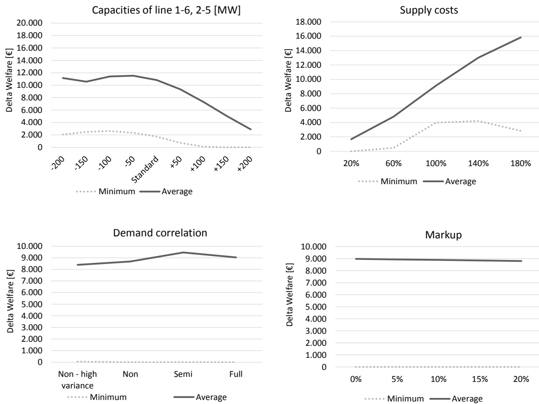
Figure 6: Delta performance of nodal to zonal pricing in the spot market
