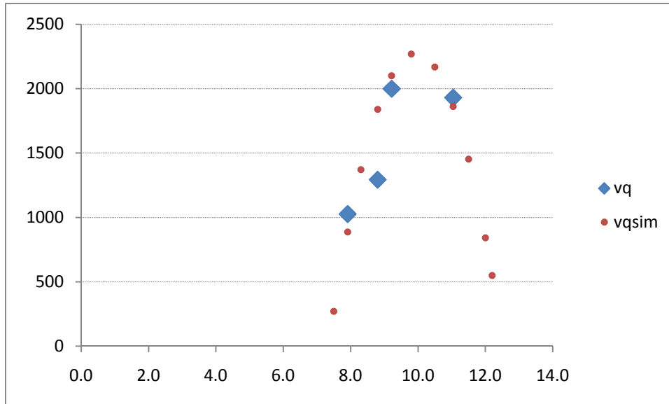
Illustration of a possible gross surplus function for a gas buyer
