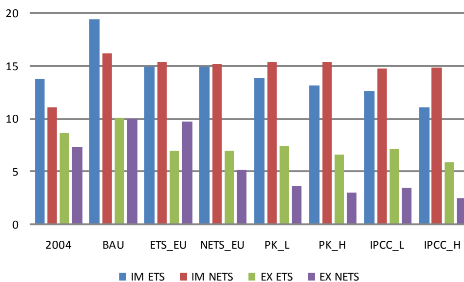
Figure 5-9: CO 2 emissions in AUT trade 2020 (Mt CO 2 )
