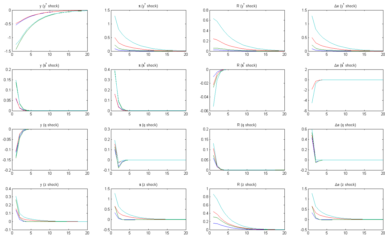
Figure 5: Impulse responses for Hungary to one-standard deviation shocks. Figure depicts the actual policy and volatility (blue), actual policy and high volatility (green), former policy and low volatility (red), and former policy and high volatility (cyan).
