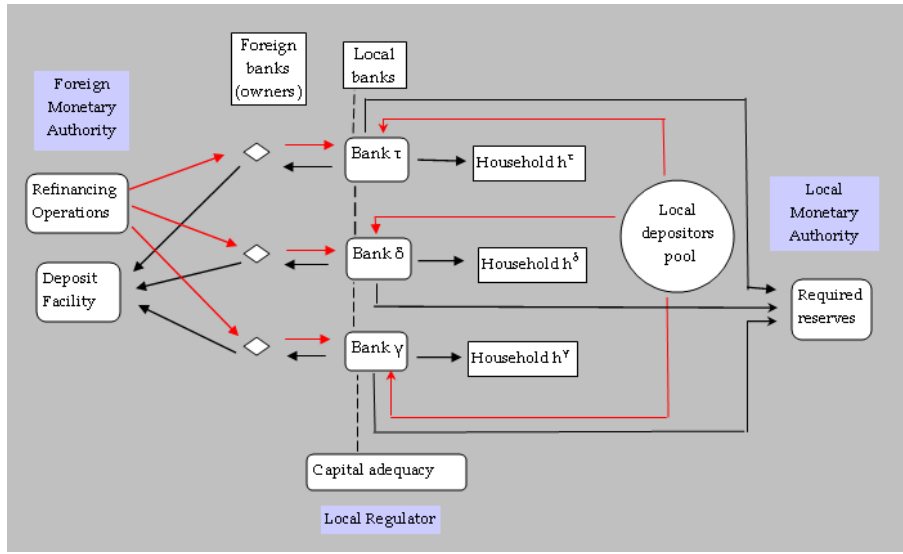
Fig. 2 Model Architecture
