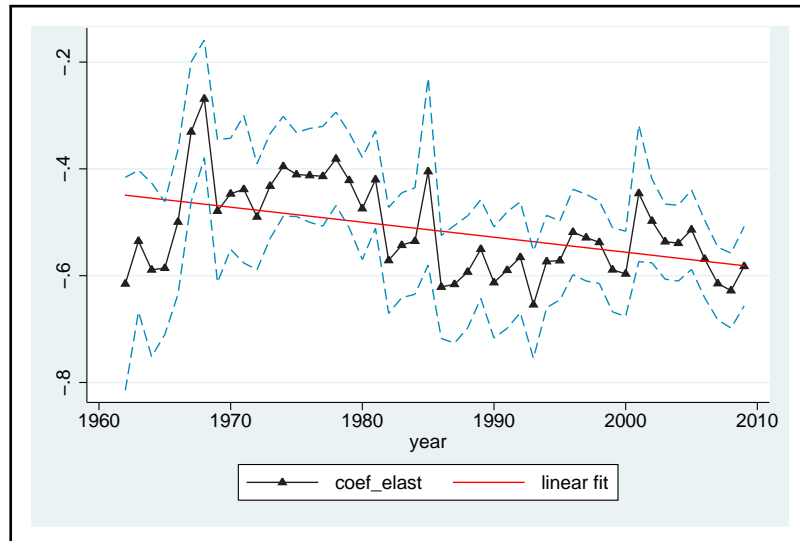
Figure 8: Estimated (1 - \tilde{\sigma})
