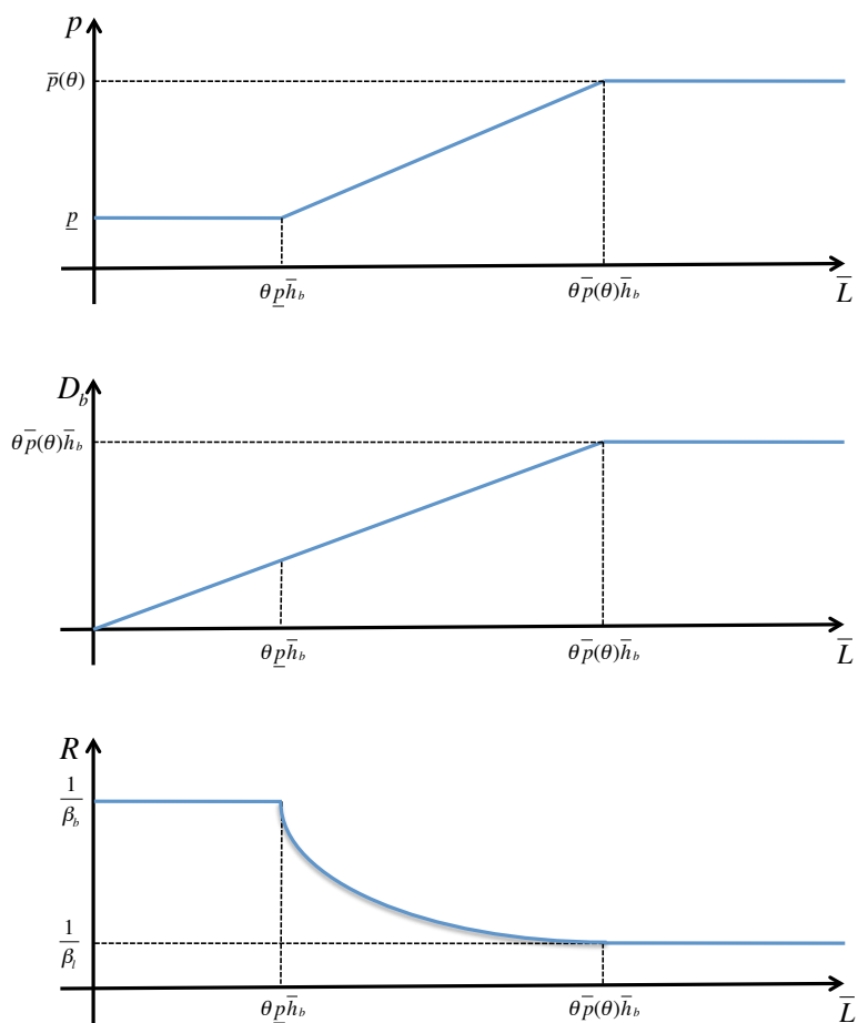
FIGURE 3.4. Real house price, debt and interest rates as a function of \bar{L} , given \theta .
