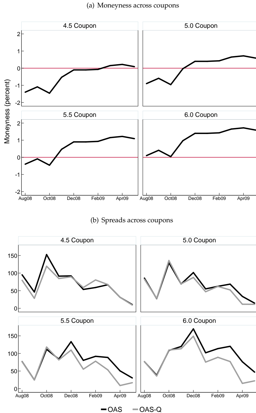
Figure 10. OAS decomposition around LSAP1 announcement This figure shows the MBS moneyiness by coupon (upper panels) and movements in OAS and OAS Q (bottom panels) based on IO/PO quotes and our prepayment model.
