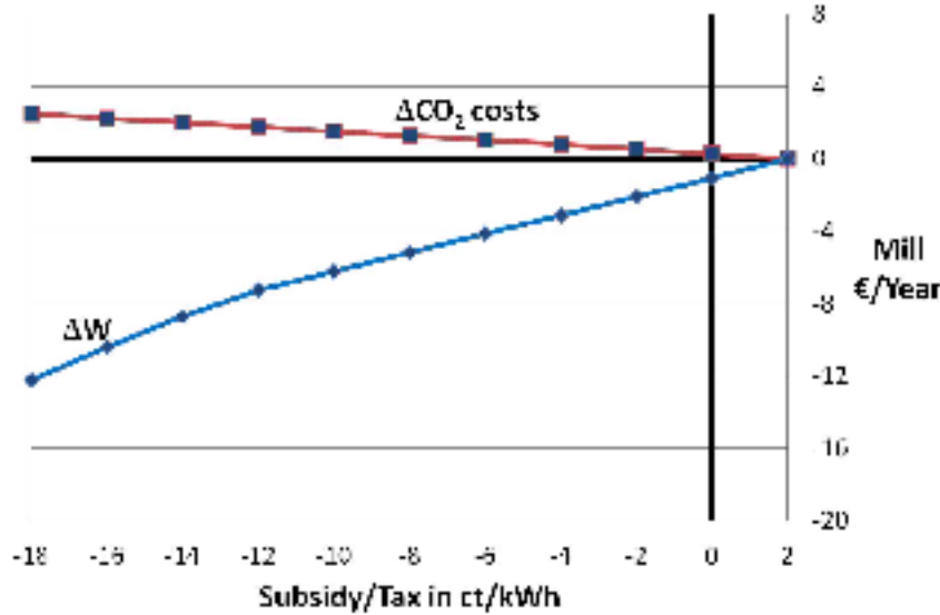
Figure 1: Baseline simulation: welfare effects and changes in emission costs
