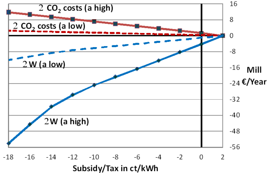
Figure 2: Welfare effects and change in emission costs for low and high responsiveness
