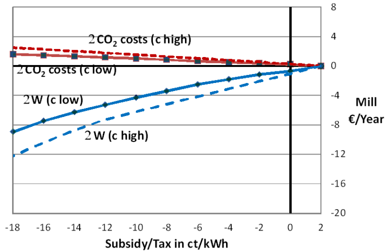
Figure 3: Welfare changes and changes in emission costs if EV's average costs per km decline.
