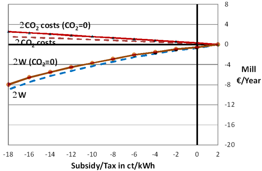
Figure 4: Change in welfare and emission costs in the case of emission trading
