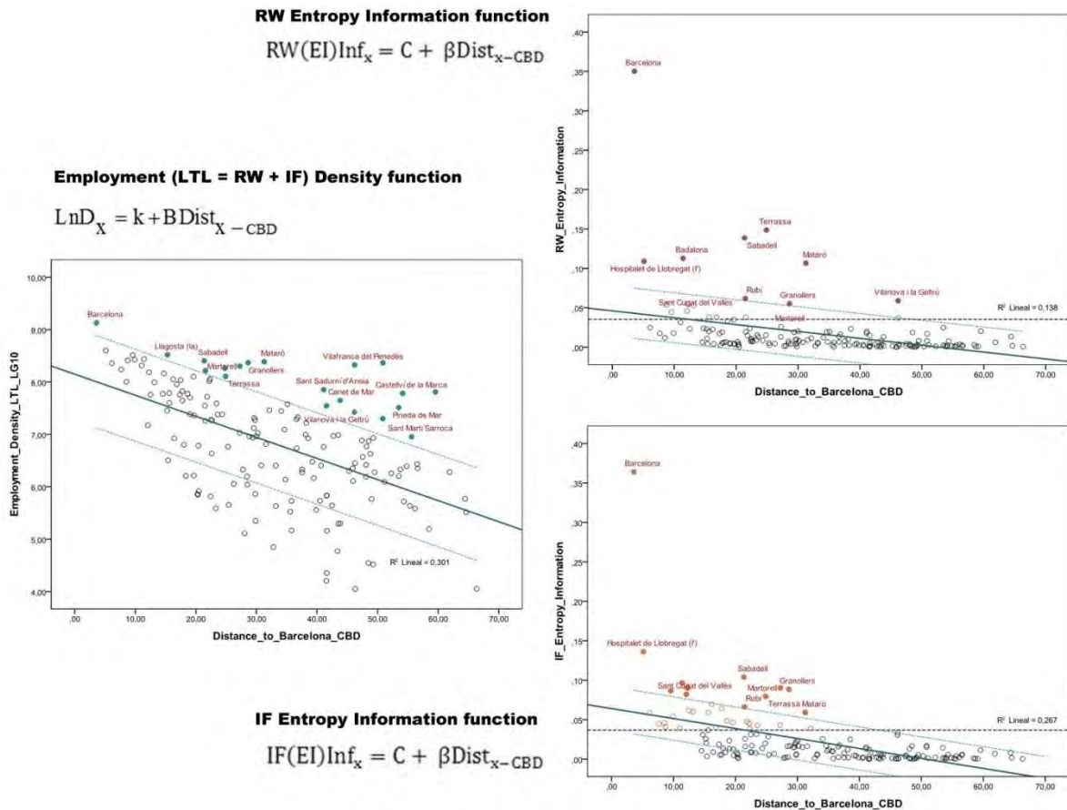
Figure 4. Employment (LTL=RW+IF) Density function versus Double Employment Entropy functions (RW and IF Entropy Information functions)
