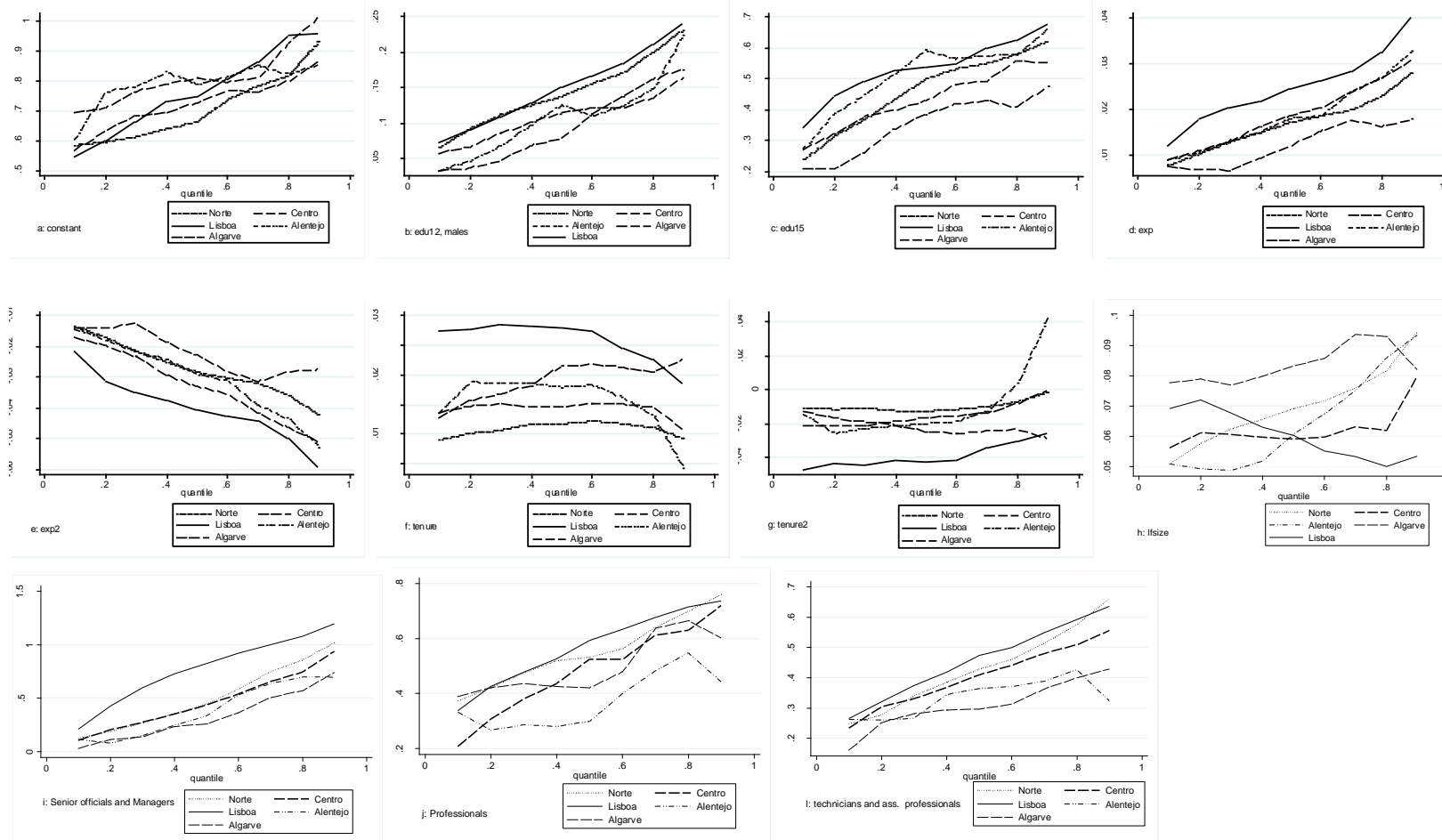
Figure 2: coeficientes estimates by quantile , males
