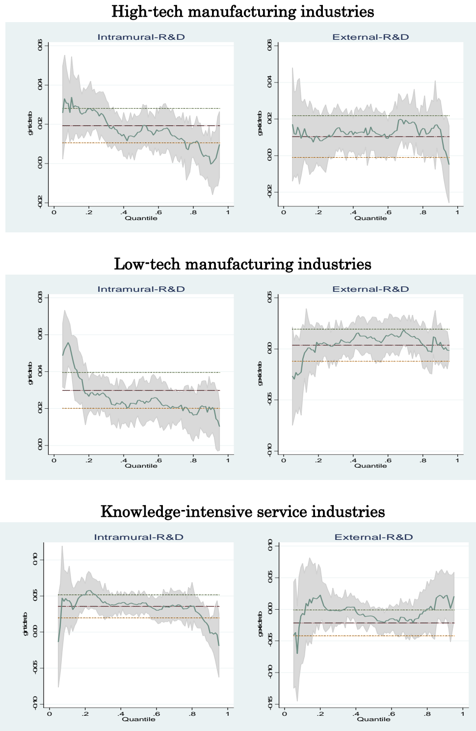
Figure 1: Marginal effects of R&D on productivity over the conditional quantiles
