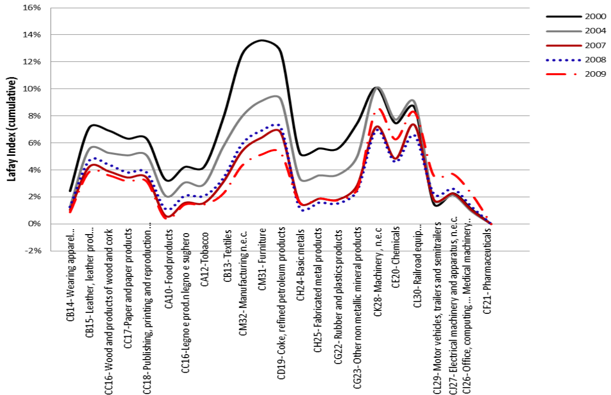
Figure 3.5 The structure of specialisation in the manufacturing industry of Toscana
