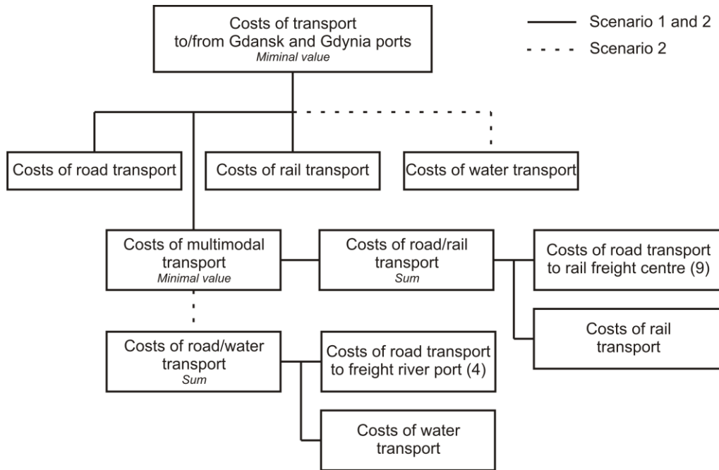
Figure 4: Data workflow
