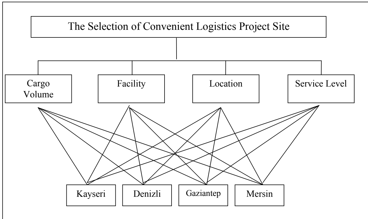
Figure 2: The Hierarchical Structure of AHP Model
