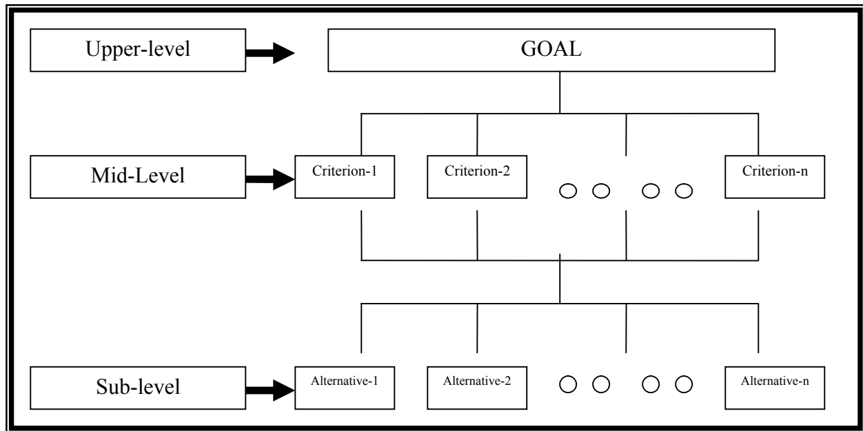
Figure 1: Hierarchical Structure of AHP
