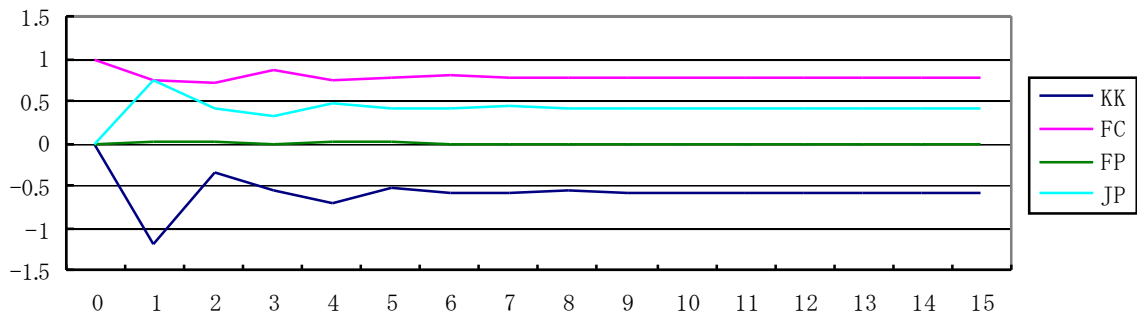
Figure 15 Impulse Response Function of VEC 3 (one unit innovations, response of FP)
