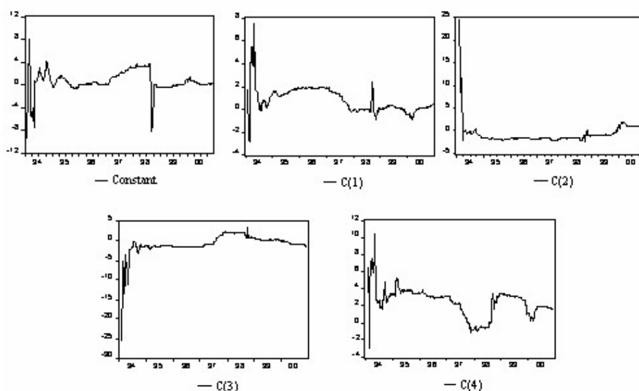
Temporal evolution of the five combination coefficients
