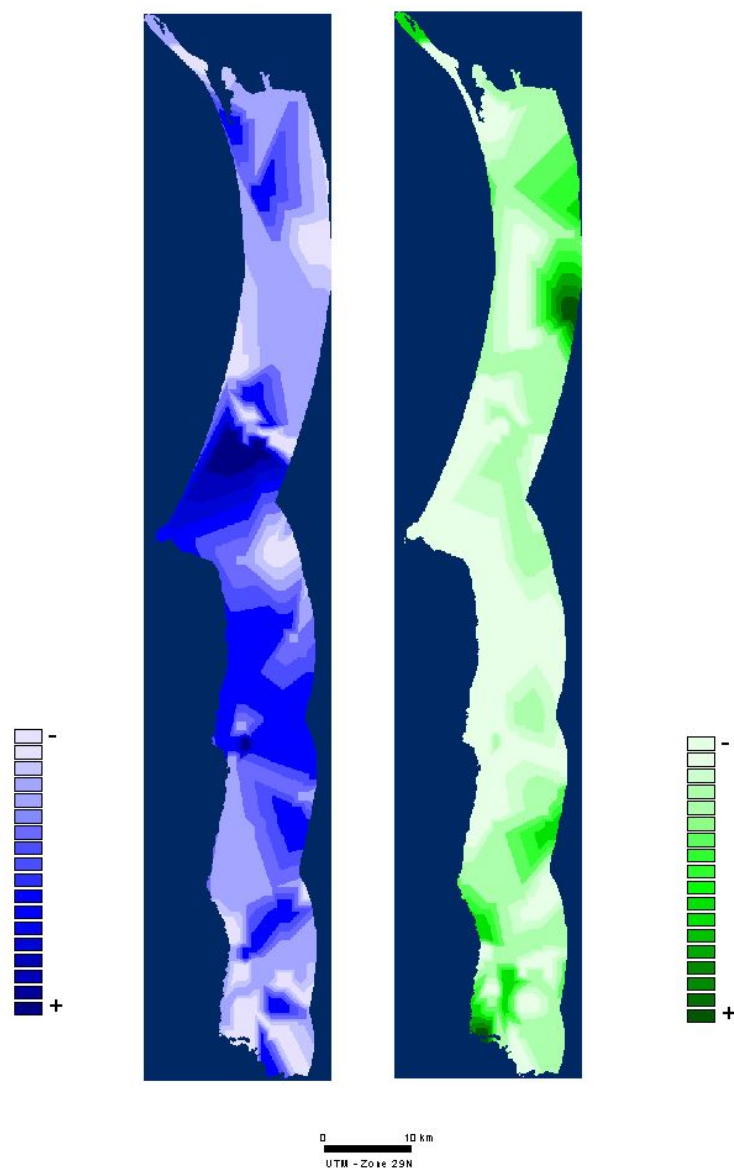
Fig. 7 – Industrial and Agro-forestry Pressure 1981-1991 in Coastal Alentejo
