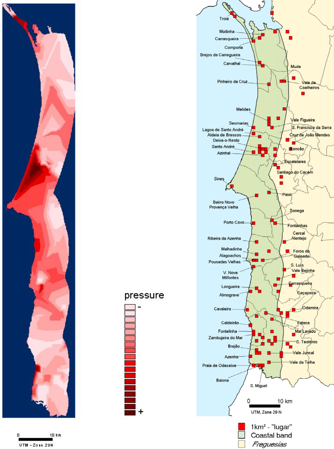
Fig. 8 – Combined Urban, Tourism and Industrial Pressure 1981-1991 in Coastal Alentejo
