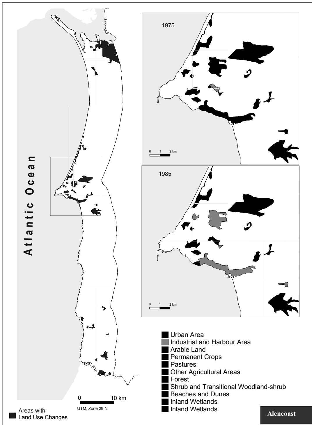
Fig. 5 – Land Cover Changes, 1975-1985, near Sines
