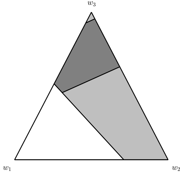
Figure 1: Support Sets on the Budget Simplex
