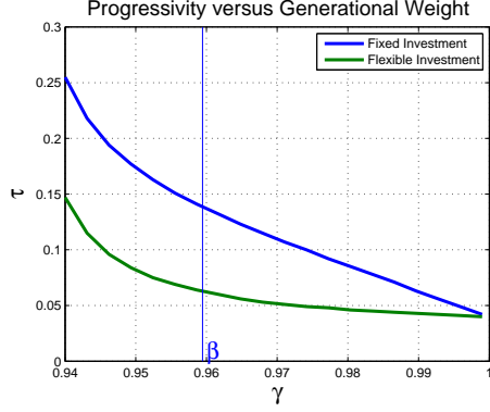
Figure 5: The figure shows how the optimal choice for \tau varies with \gamma in the baseline flexible (reversible) investment model and the alternative fixed (irreversible) investment model.
