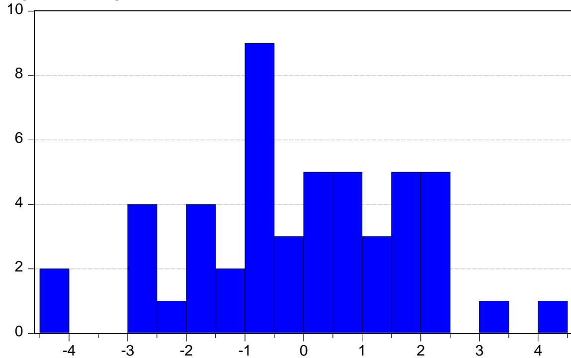
Figure 1: Histogram of differences between Irish and UK inflation rates, 1923-1979
