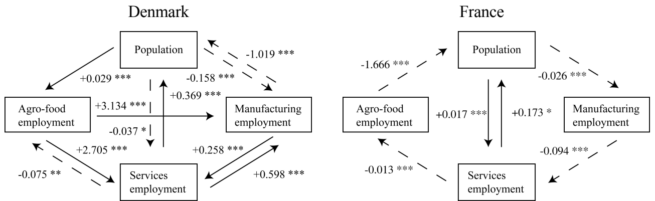
Figure 2. Dynamic externalities (W+I).X_{t-1}
