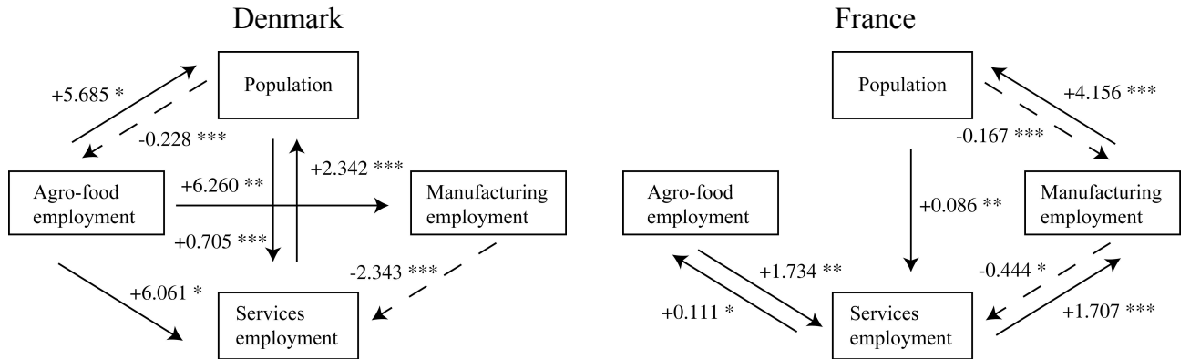
Figure 1. Static externalities (W+I).\Delta X_t
