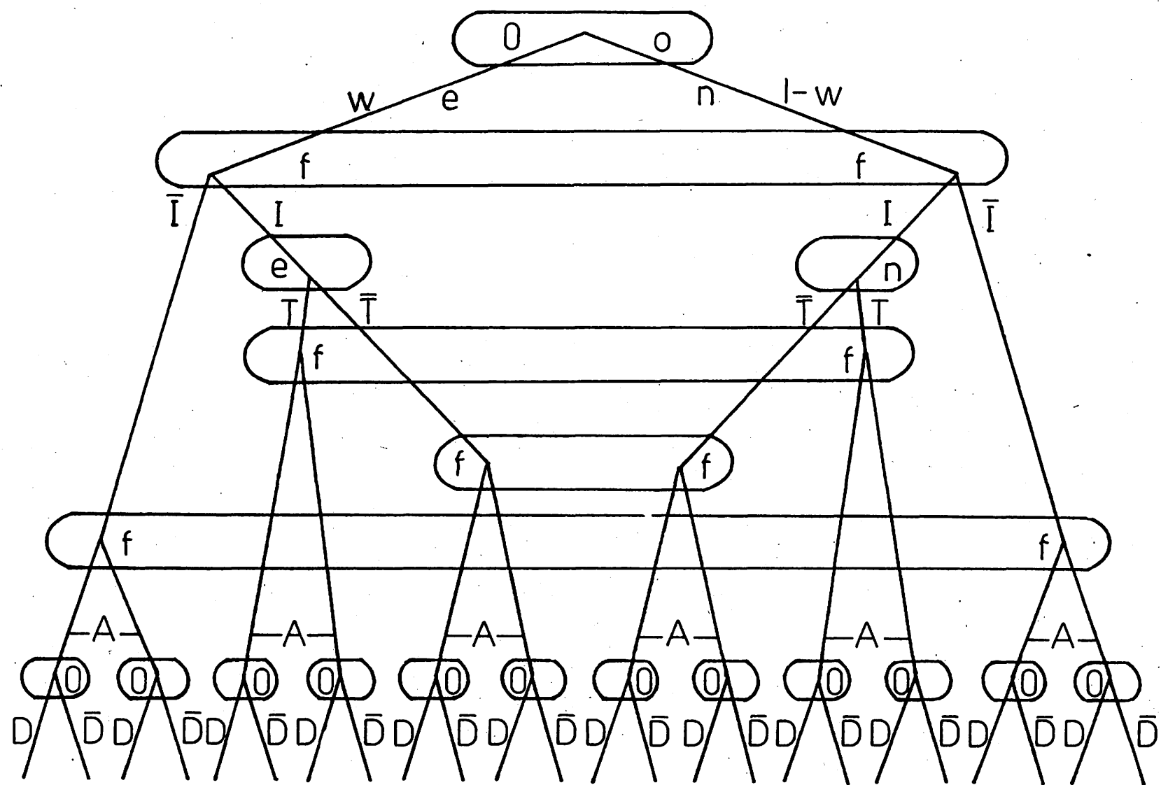
Figure 2.1: The game tree of the game model.
