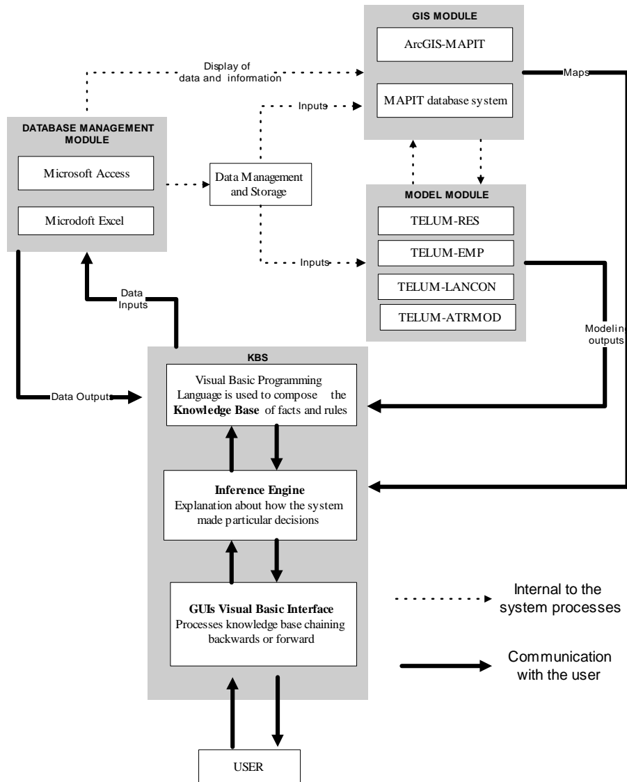
Fig. 2. TELUM Structural Overview
