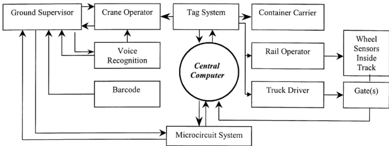
Figure 4 – Management System Architecture
