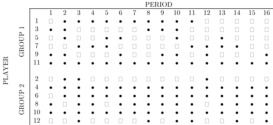
Figure 2a: The choices of players in each period. The symbol • indicates a player chose H and □ indicates that a player chose D.
