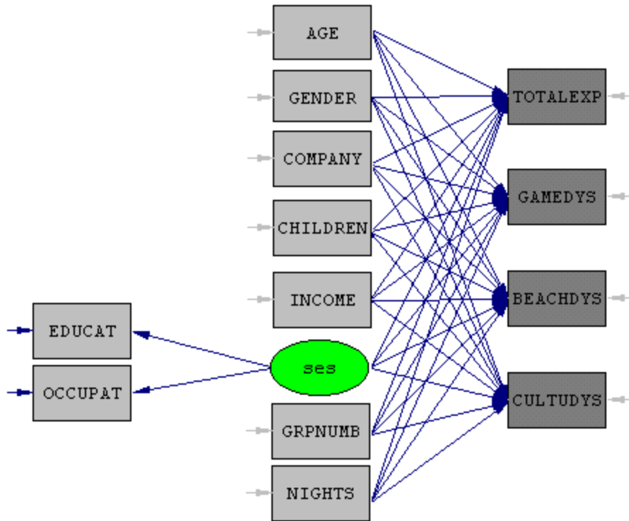
Figure II: Path Diagram
