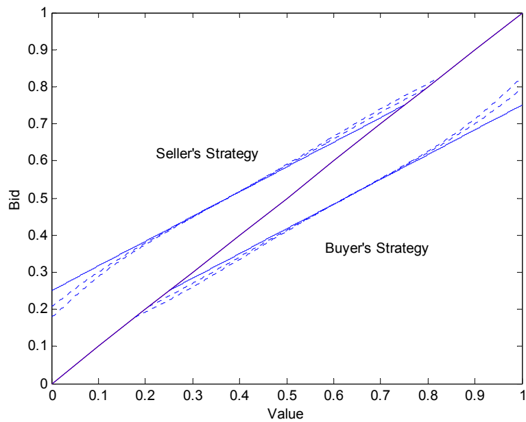
Figure 4: Convergence to the Linear Equilibrium
