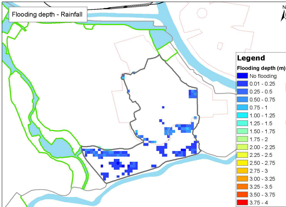
Figure 7: Overview of the inundation depths in the study area by flooding caused by lack of discharge capacity due to extreme rainfall.
