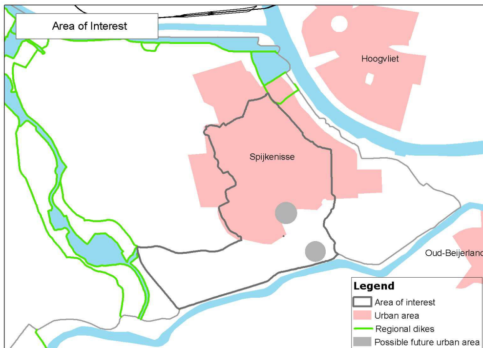
Figure 8. Two possible future urban areas are located on the map. The most Northern location gives only a small increase in flood risk, whereas the more southern location leads to a relative large increase in flood risk by regional flood defences.
