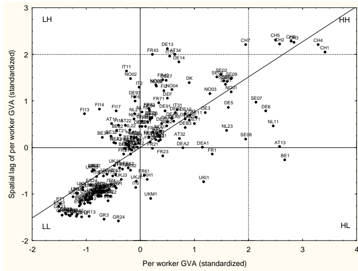
Figure 4: Moran scatterplot for GVA per worker in 1977
