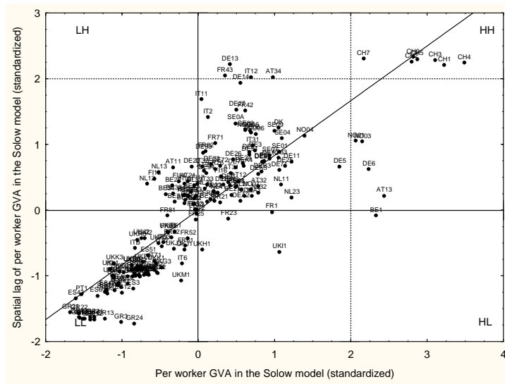
Figure 7: Moran scatterplot for GVA per worker implied by the spatial Solow model
