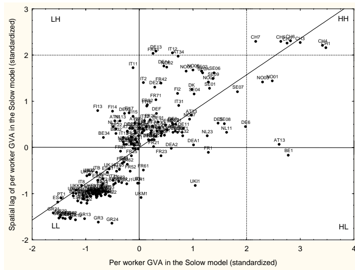
Figure 6: Moran scatterplot for GVA per worker implied by the Solow model
