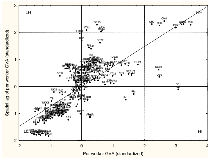
Figure 5: Moran scatterplot for GVA per worker in 2000
