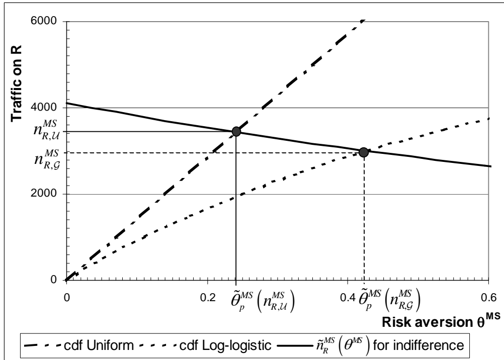
Figure 3: Equilibrium for MS preferences with uniform and log-logistic distributions for risk aversion
