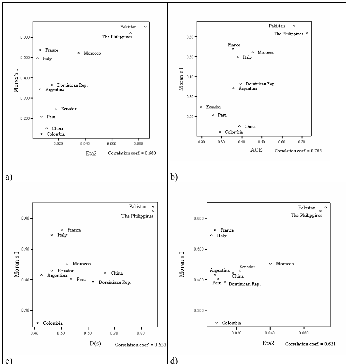
Figure 3. Scatter plots between segregation measures and Moran's I, only significant correlation coefficients.
