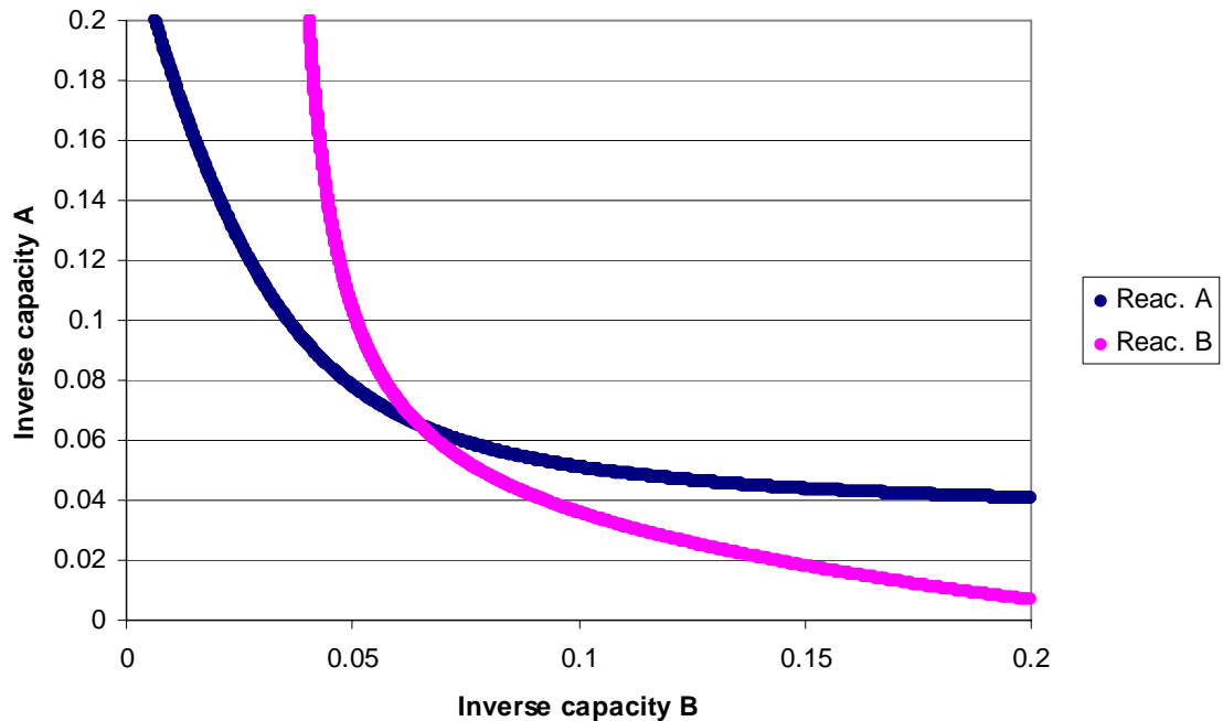
Figure 1 Inverse capacity reaction functions for the Nash equilibrium of the central scenario
